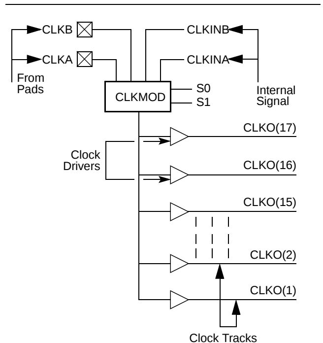
Figure 7 • Clock Networks
