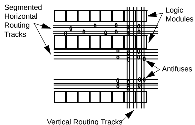
Figure 6 • Routing Structure
